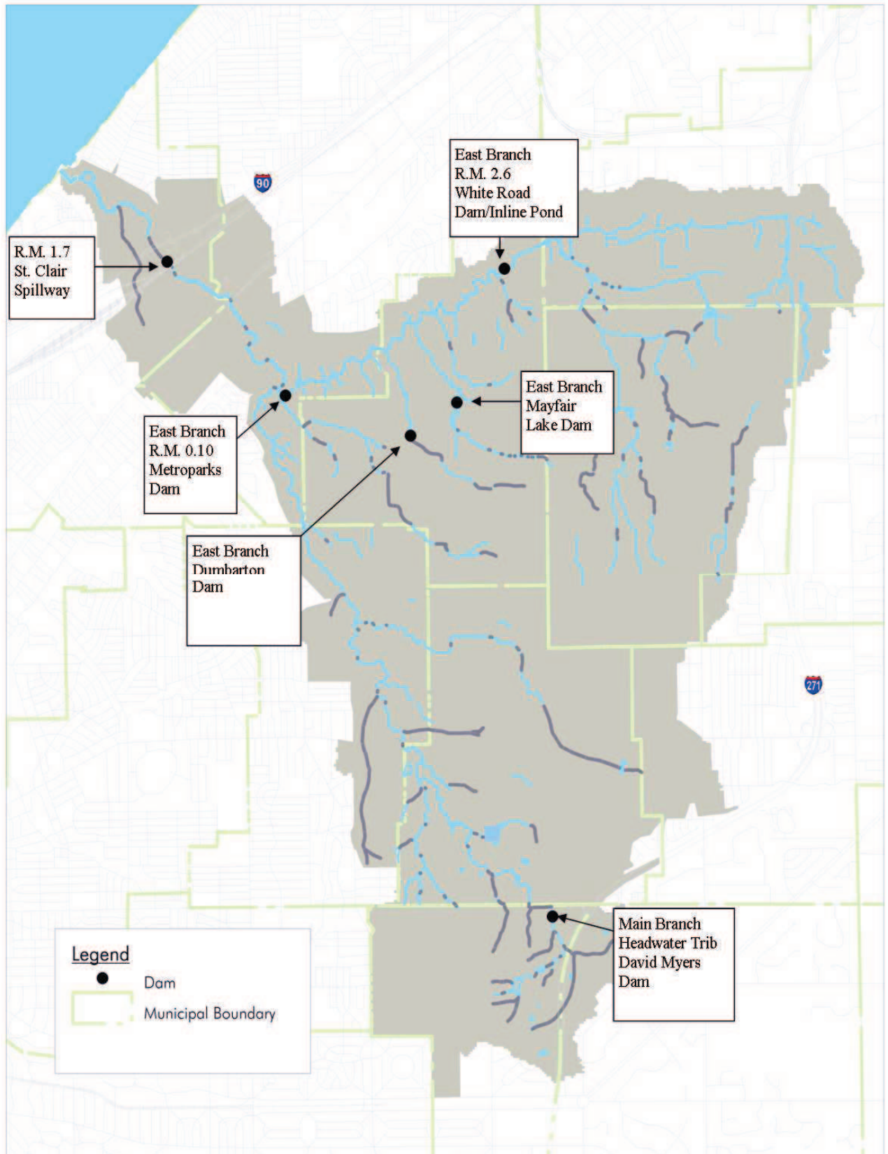
Figure 39. Dam Locations in Euclid Creek Watershed
